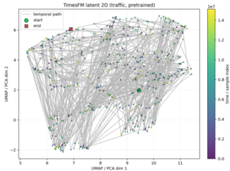
Traffic
