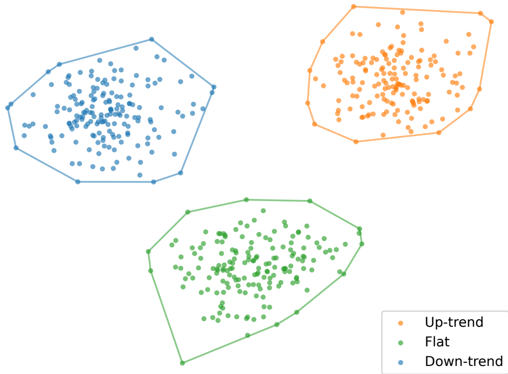
Pretrained (LCS = 0.000)
