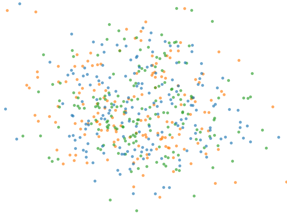
Random (LCS = 0.000)
