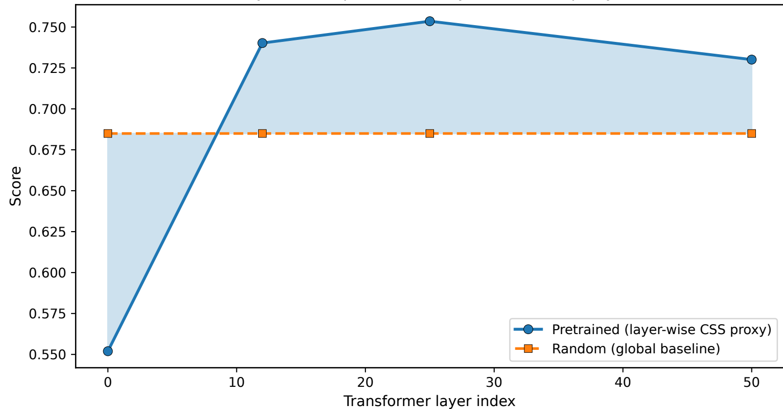
Layer-wise representation dynamics (CSS proxy)
