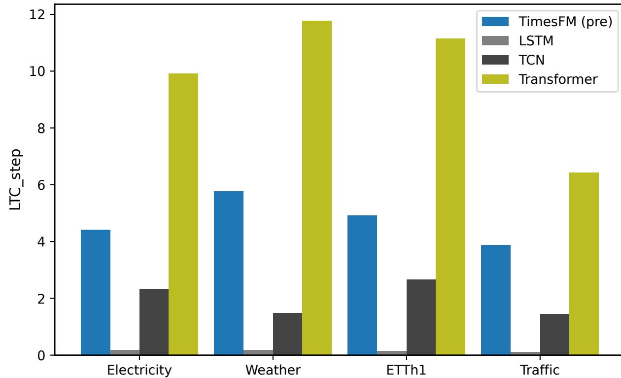
Across datasets
