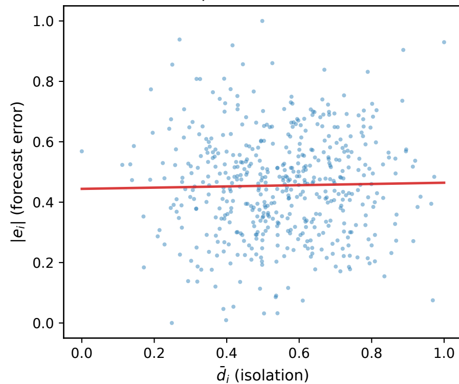
CSI300 \rho = 0.22 ***
