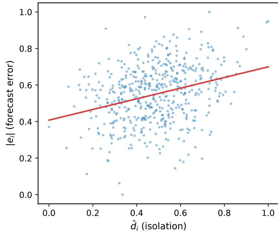
Traffic \rho = 0.27 ***
