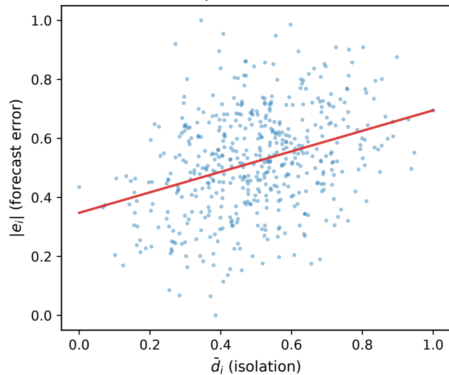
Traffic \rho = 0.27 ***
