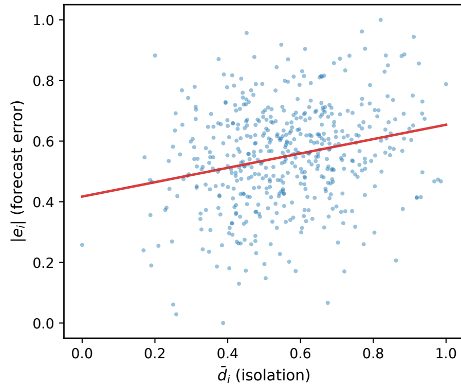
CSI300 \rho = 0.22 ***
