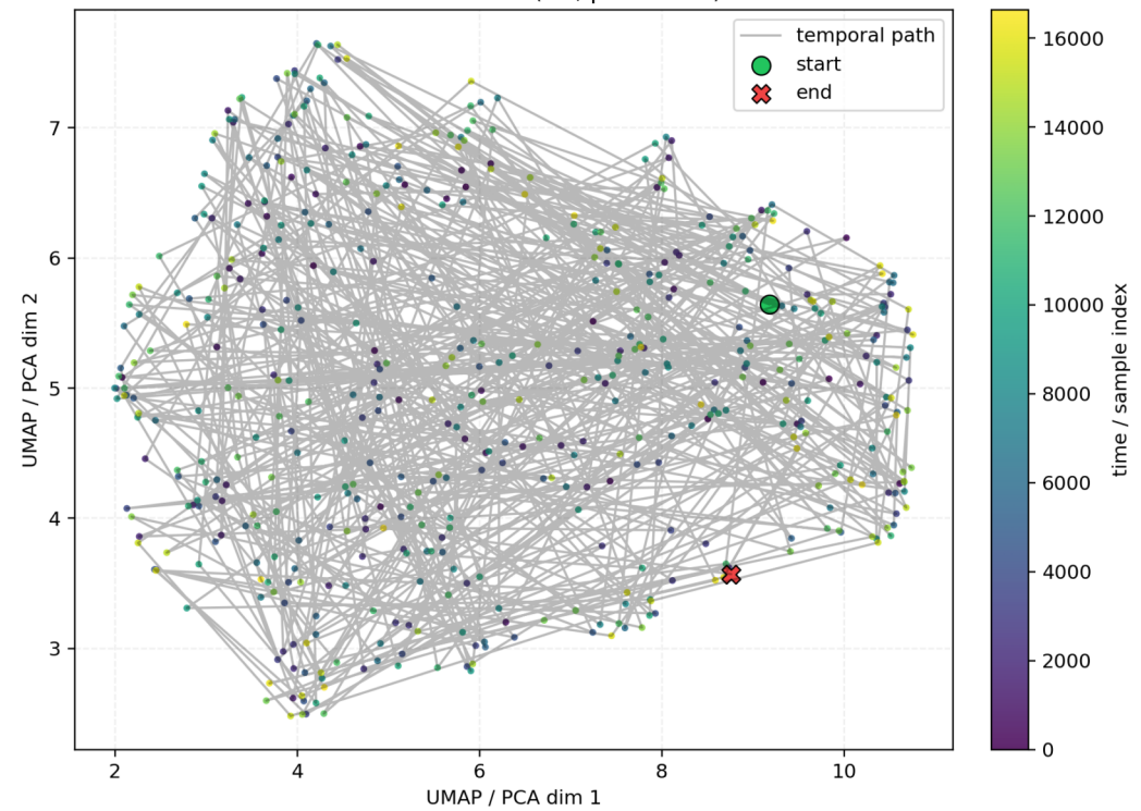
TimesFM latent 2D (ett, pretrained)
