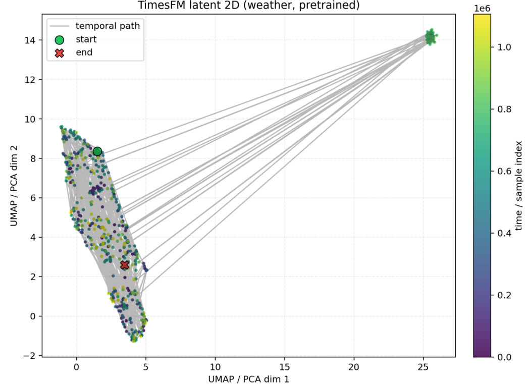
TimesFM latent 2D (weather, pretrained)
