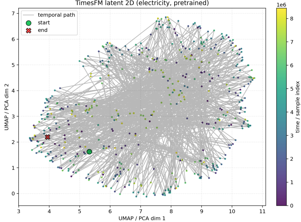
TimesFM latent 2D (electricity, pretrained)
