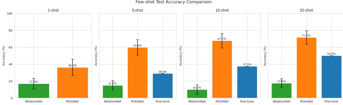
Figure 9: Few-shot test accuracy comparison. Error bars represent standard deviation (ProtoNet, RelationNet). Fine-tune results are single runs.
