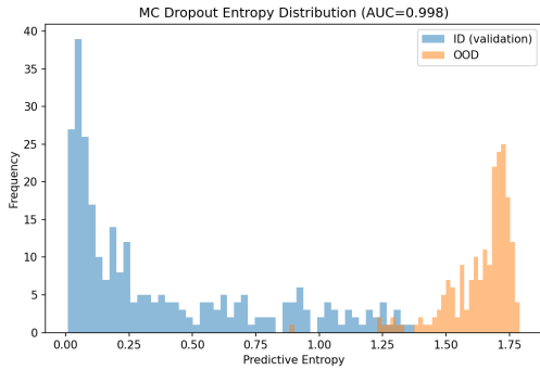
Figure 10: Entropy distribution on far OOD (random internet images). ID samples concentrate at very low entropy, OOD samples at high entropy, with almost no overlap.
