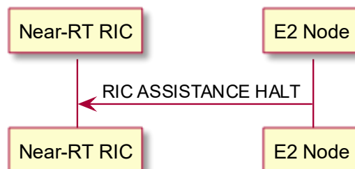
Figure 8.2.13.2-1: RIC Assistance Halt procedure, successful operation
