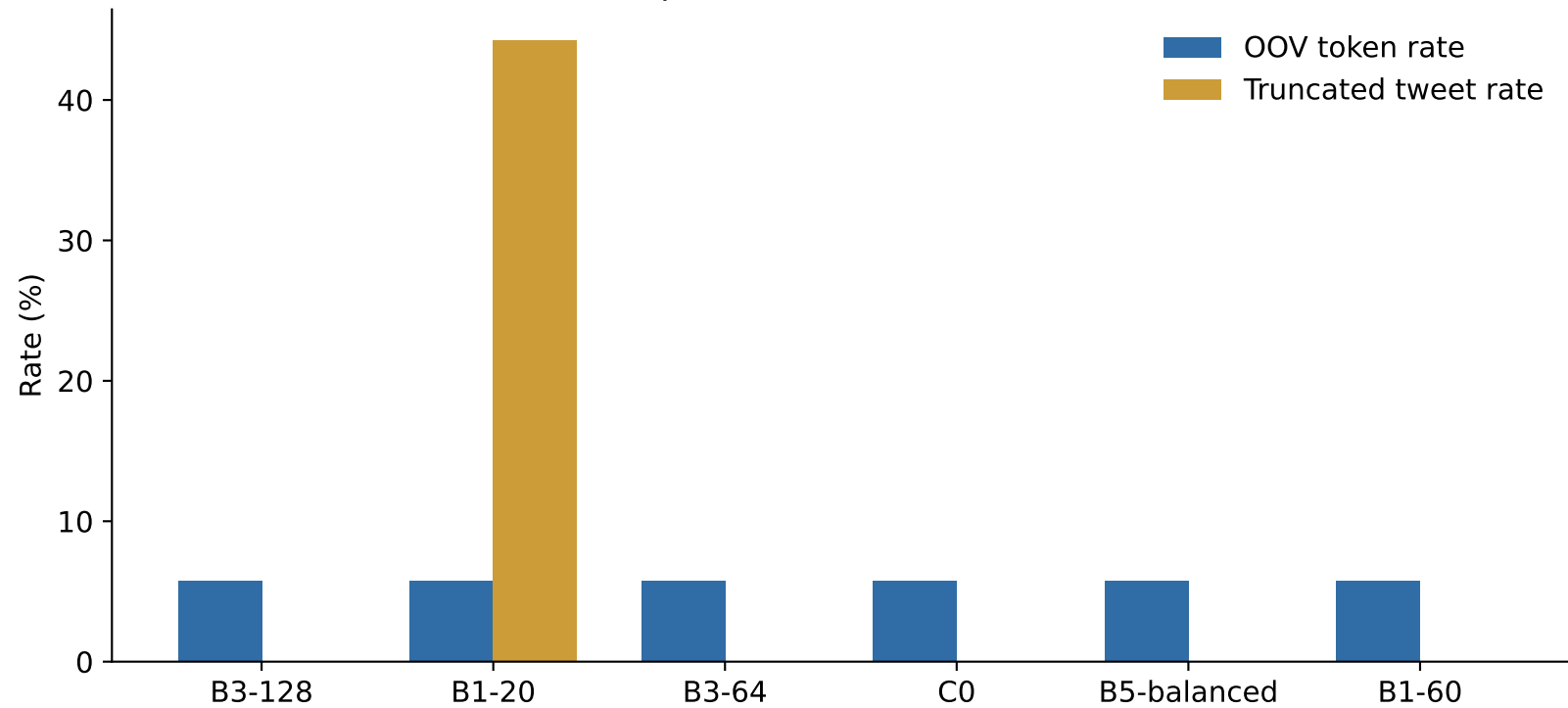
Validation representation: OOV and truncation
