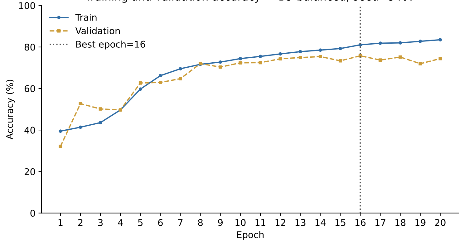
Training and validation accuracy — B5-balanced, seed=3407
