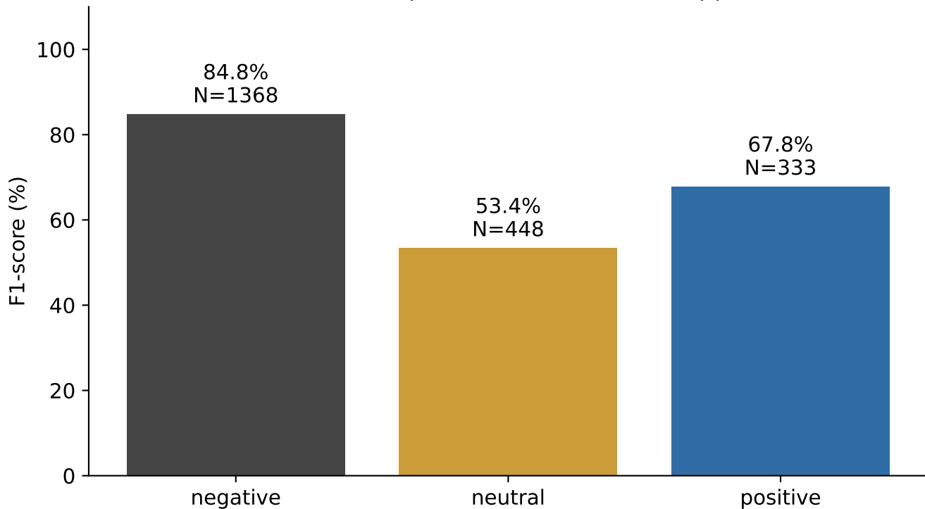
Final model: per-class test F1 and support
