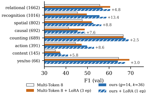
(b) By reasoning type (gain of ours + LoRA over Multi-Token 8)
