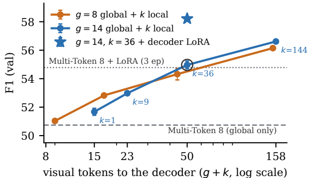
(a) Accuracy against visual tokens
