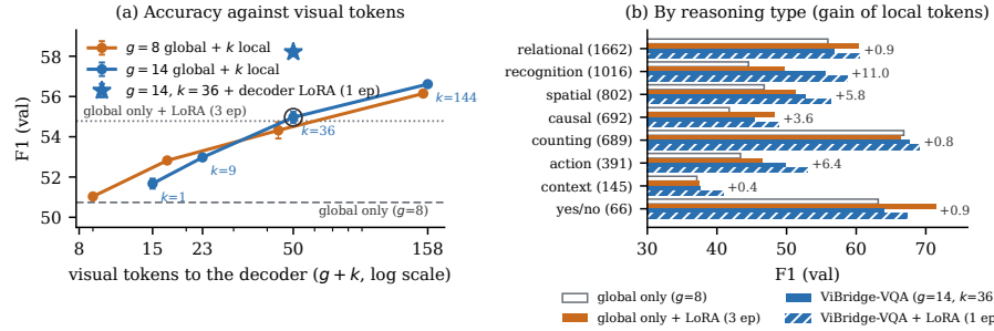
Fig. 2: (a) Validation F1 against the number of visual tokens (mean \pm std over three seeds); the circled point is the knee, g = 14, k = 36 . Horizontal lines: the global-only model (four seeds) and the same model with a three-epoch decoder LoRA (three seeds). (b) Validation F1 by reasoning type (number of questions in parentheses), each model averaged over all of its seeds (global only: four; others: three); the numbers give the gain of ViBridge-VQA ( g = 14, k = 36 , no LoRA) over the global-only model ( g = 8 ).
