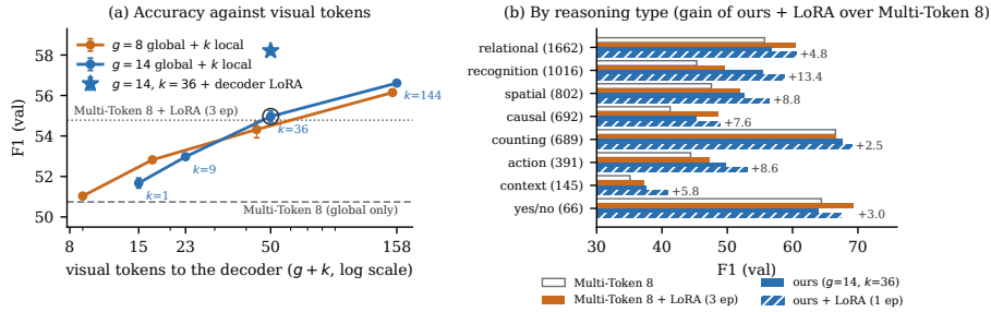
Fig. 2: (a) Validation F1 against the number of visual tokens (mean \pm std over 3 seeds); the circled point is the knee, g = 14 , k = 36 . Horizontal lines: the global-only Multi-Token model (4 seeds) and the same model with a 3-epoch decoder LoRA (3 seeds). (b) Validation F1 by reasoning type (number of questions in parentheses): global only and + LoRA for seed 42, ViBridge-VQA ( g = 14 , k = 36 ) without and with a 1-epoch decoder LoRA averaged over 3 seeds; numbers are the gain of ViBridge-VQA + LoRA over the global-only model.
