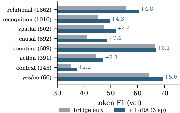
(b) Gain by reasoning type
