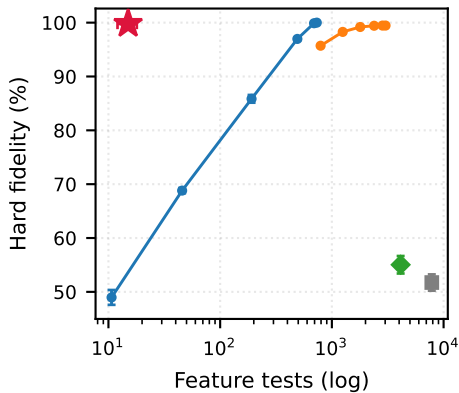
Pong
