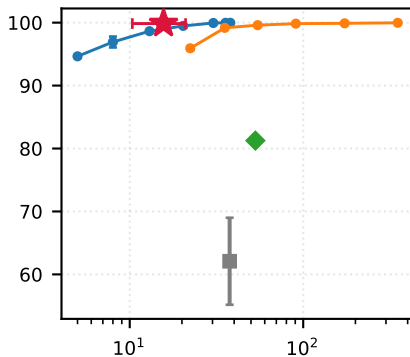
Boxing
