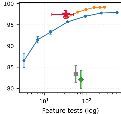
PixelCartPole
