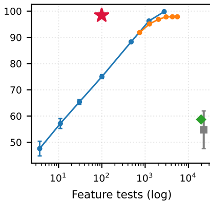
Boxing
