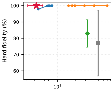
Pong
