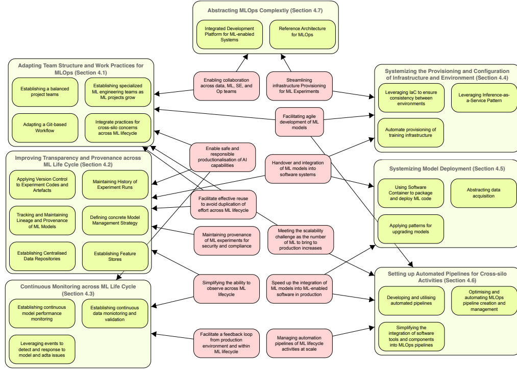
Fig. 4. MLOps practices and techniques, and the corresponding ML productionalization challenges
