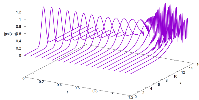
(c) k_0 = 10 .
