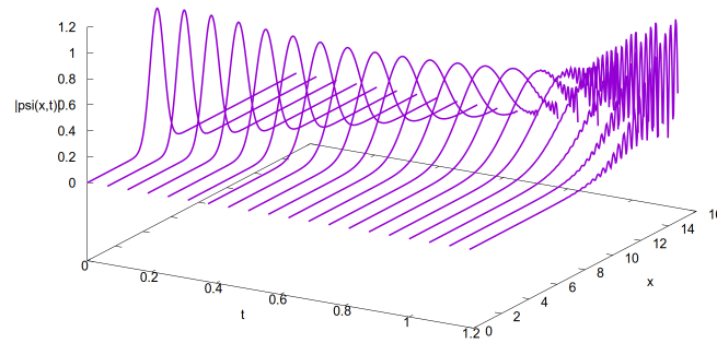
(b) k_0 = 8 .
