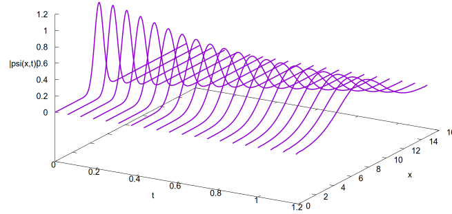
(a) k_0 = 2 .
