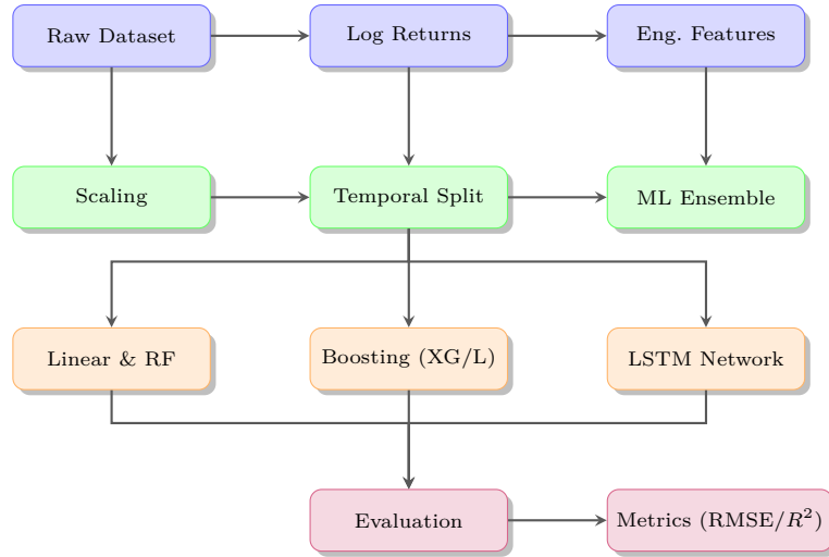
Fig. 1: Premium research methodology workflow for housing price prediction.
