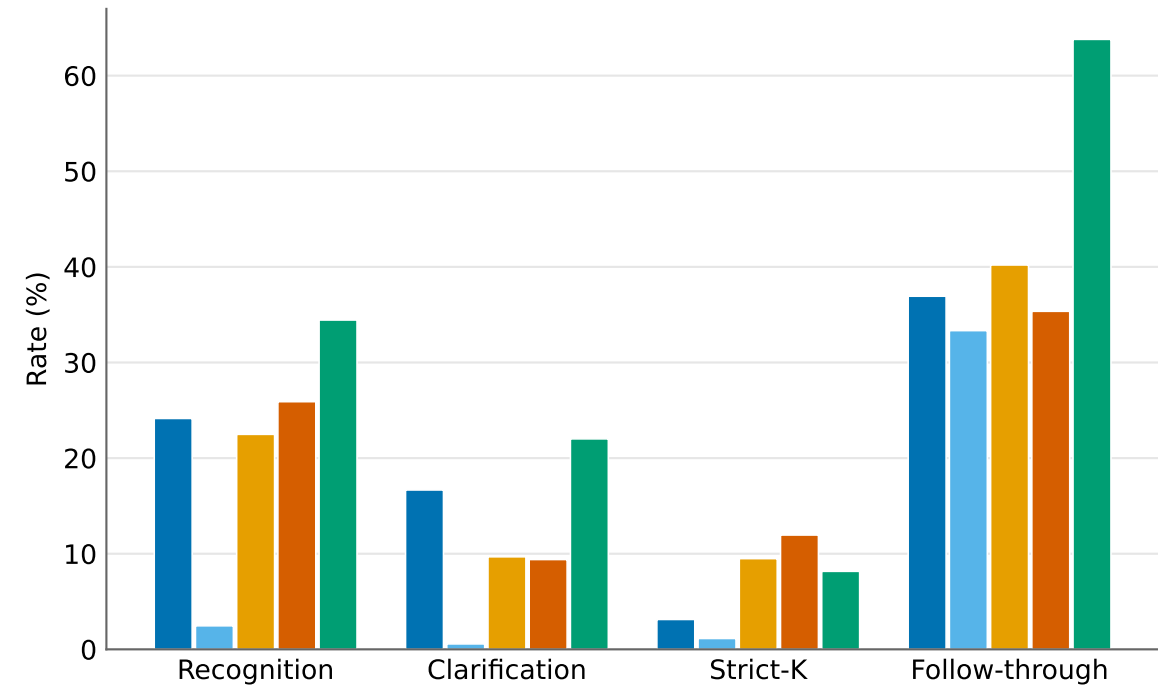
Behavioral metric breakdown
