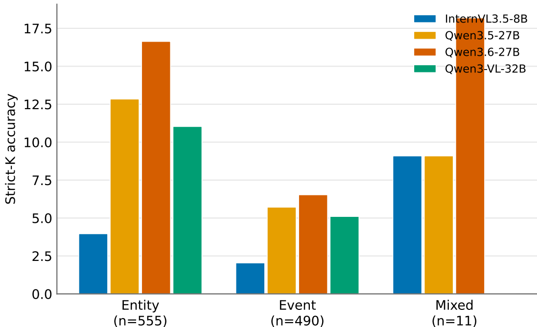
Strict-K accuracy by ambiguity type
