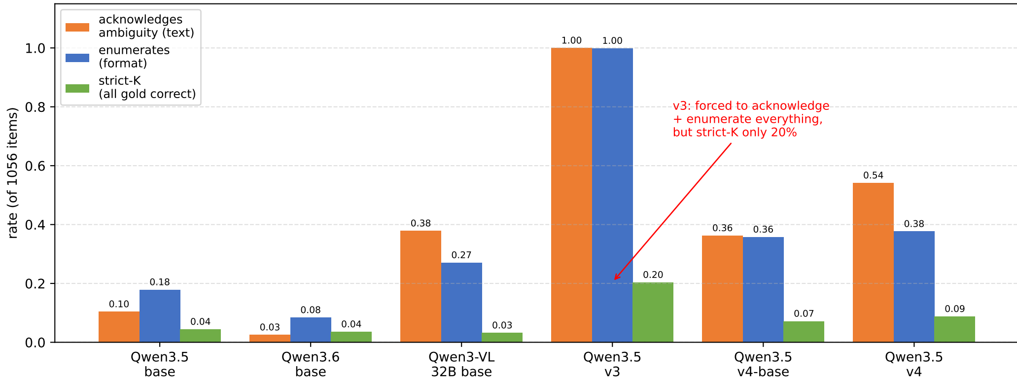
Format >> substance: across configs, strict-K stays low while format inflates
