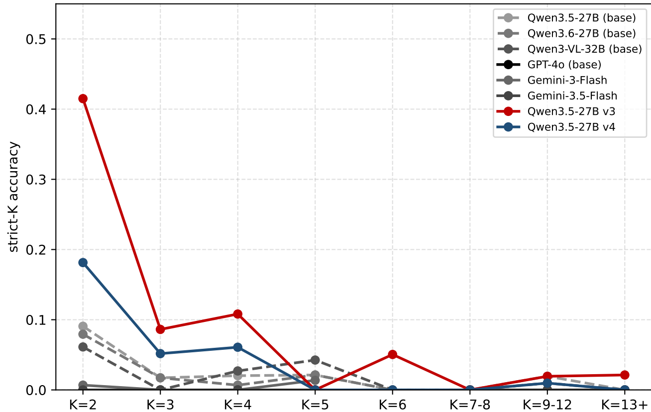
(a) Strict-K accuracy by K
