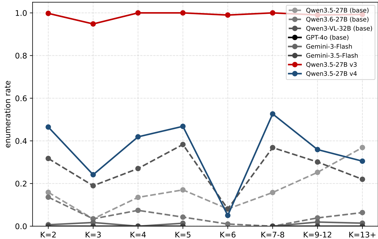
(b) Enumeration rate by K
