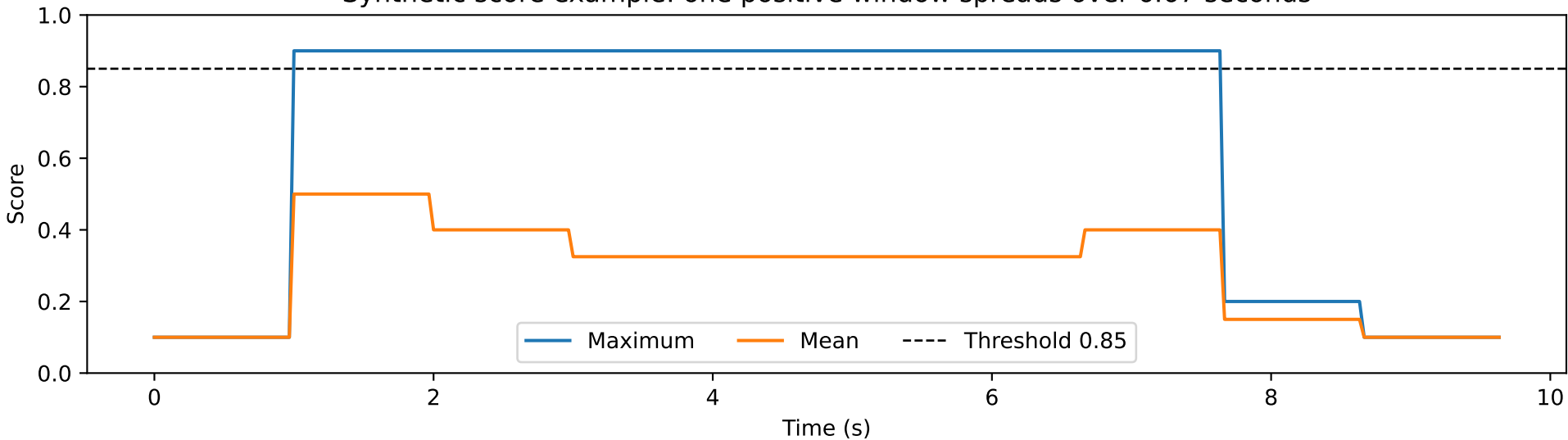
Synthetic score example: one positive window spreads over 6.67 seconds
