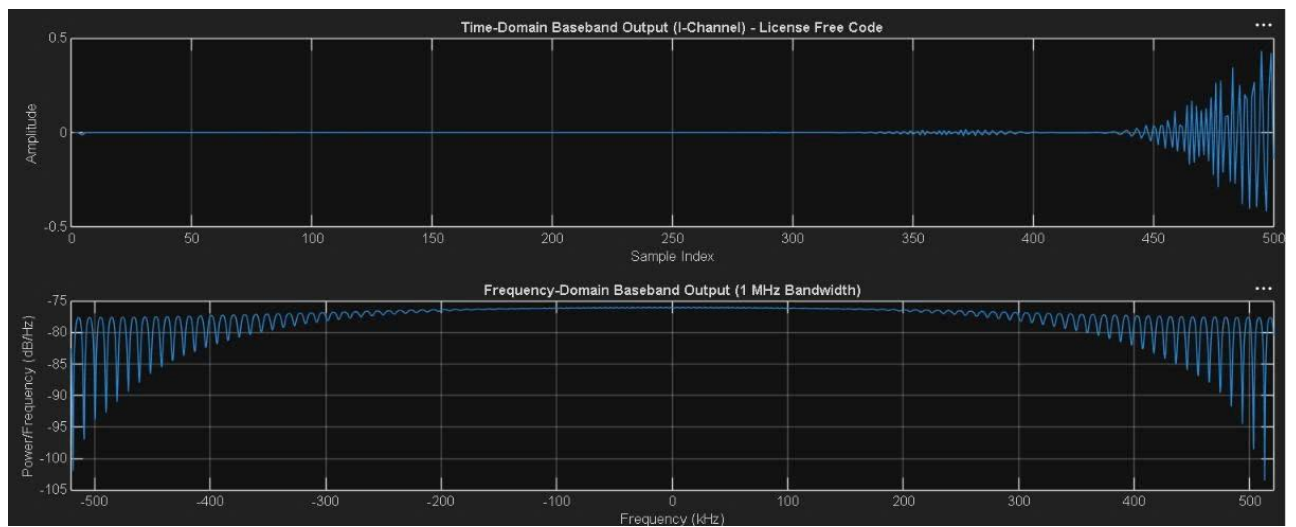
Figure 4.2: Time-Domain and Frequency-Domain Response of the Math-Quantized DDC Output
