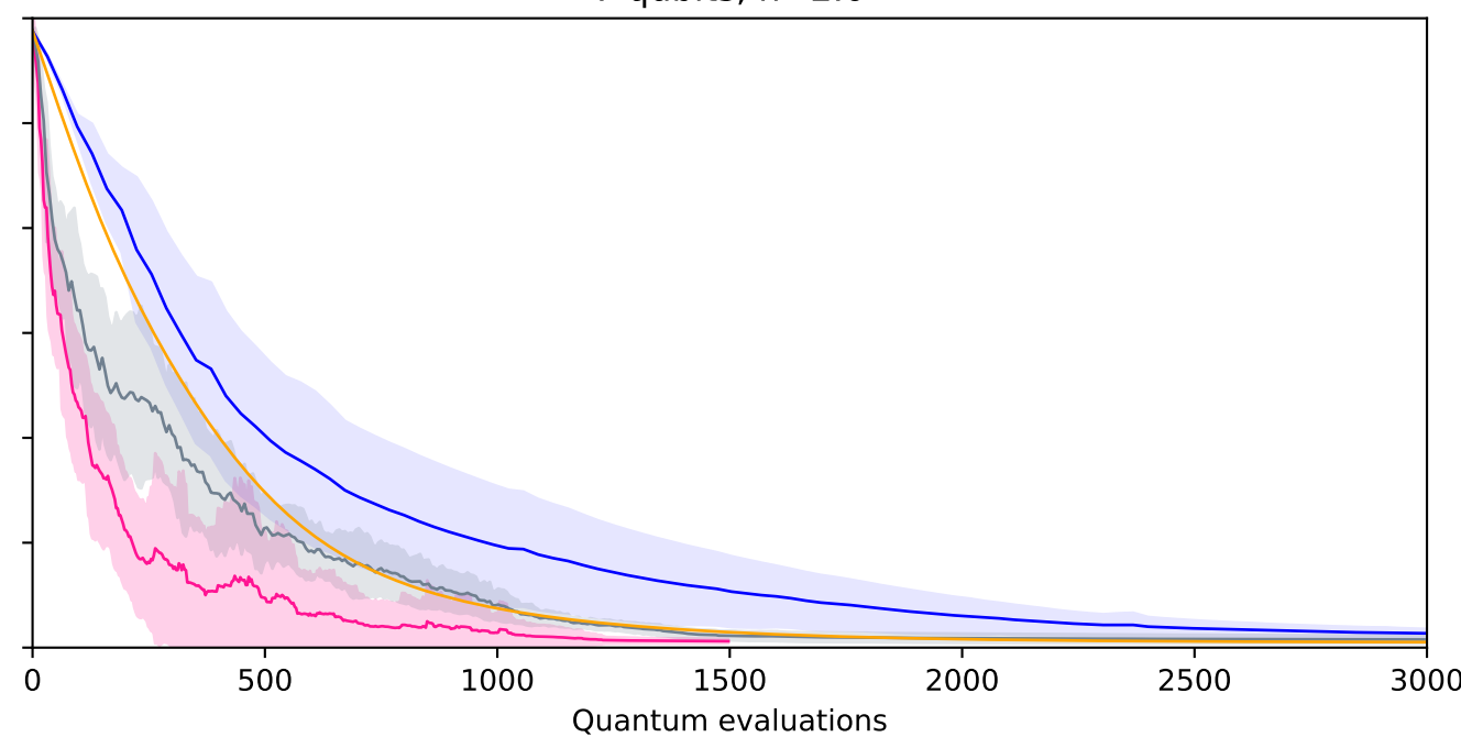
7 qubits, h=2.0
