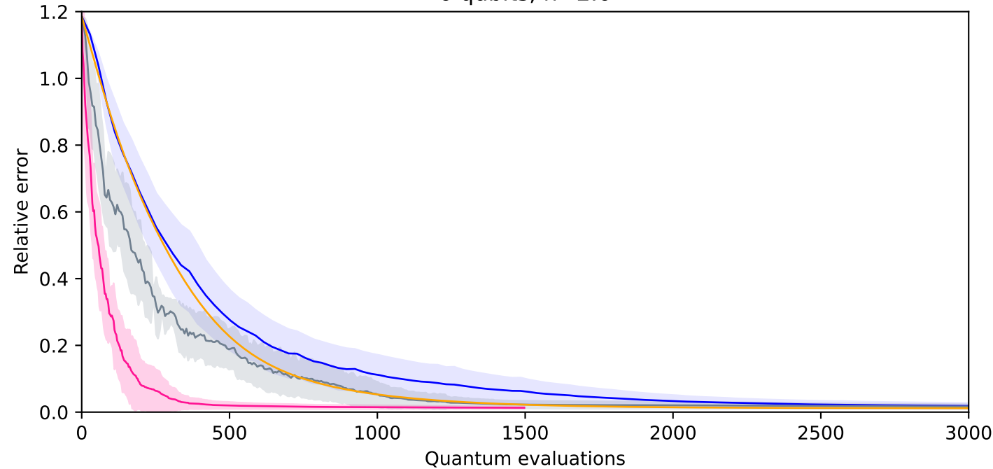
6 qubits, h=2.0
