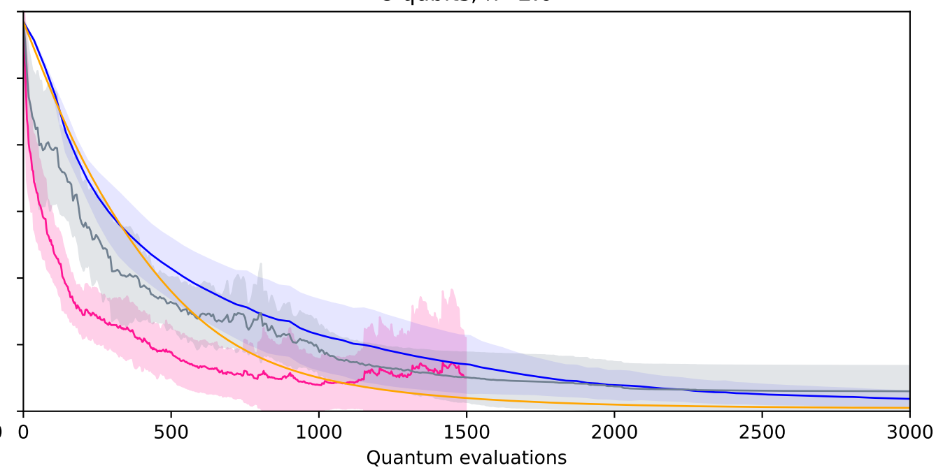
8 qubits, h=2.0
