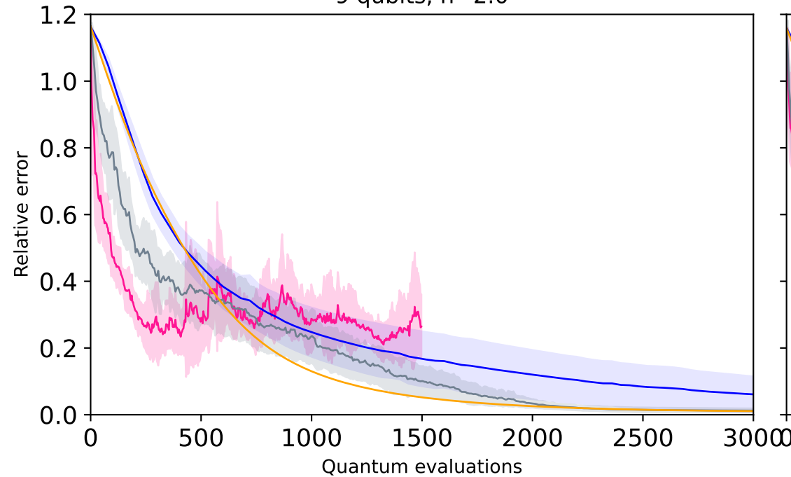
9 qubits, h=2.0
