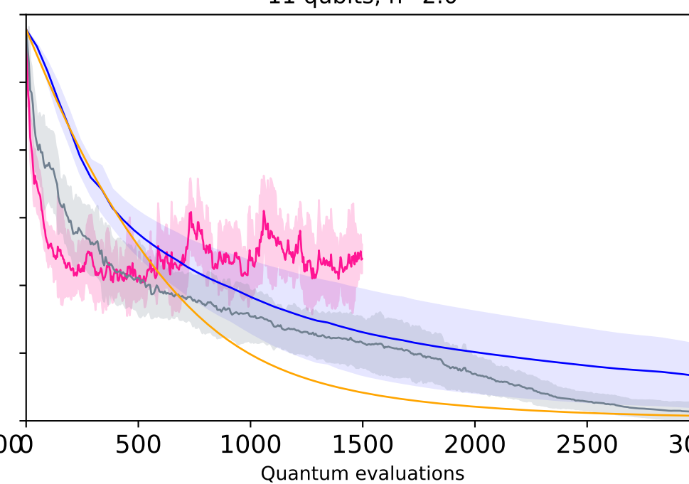
11 qubits, h=2.0
