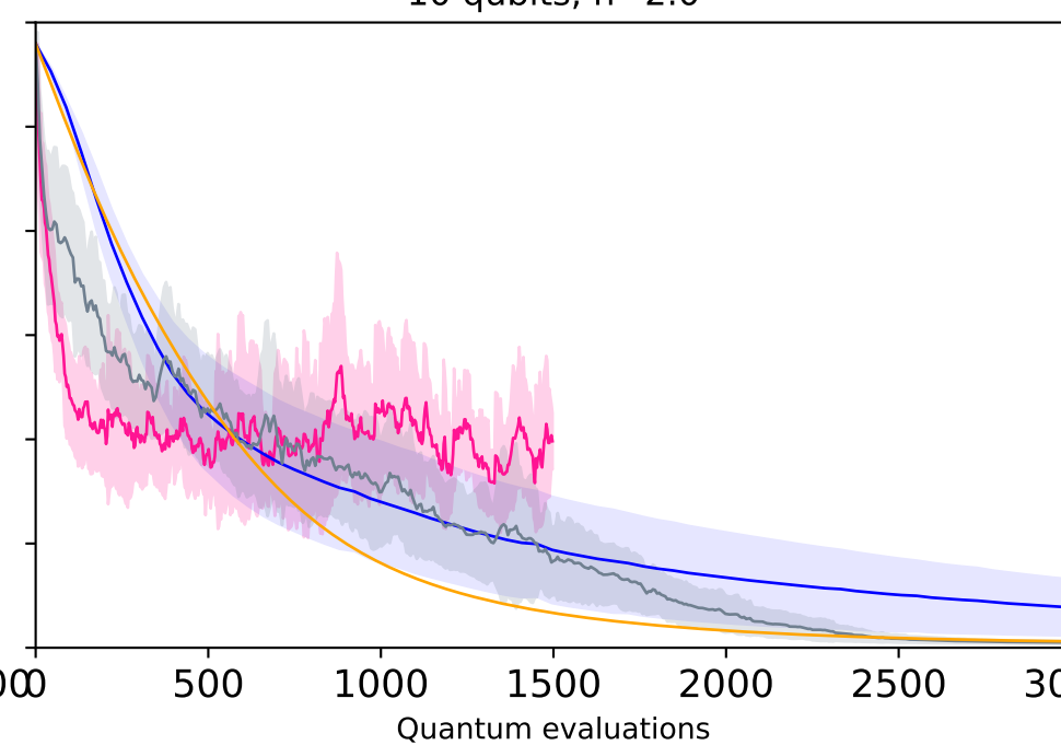
10 qubits, h=2.0
