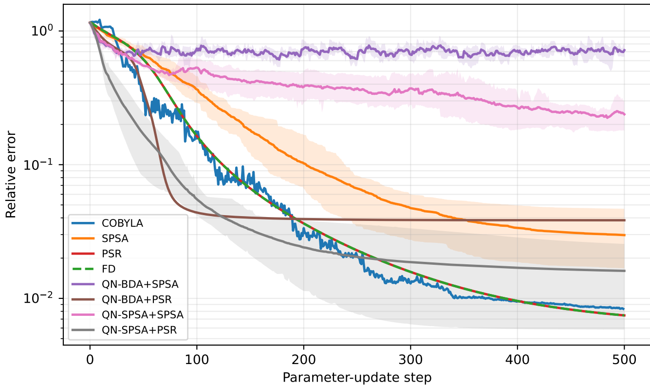
RealAmplitudes, n=11 , h=2.0 , reps=2
