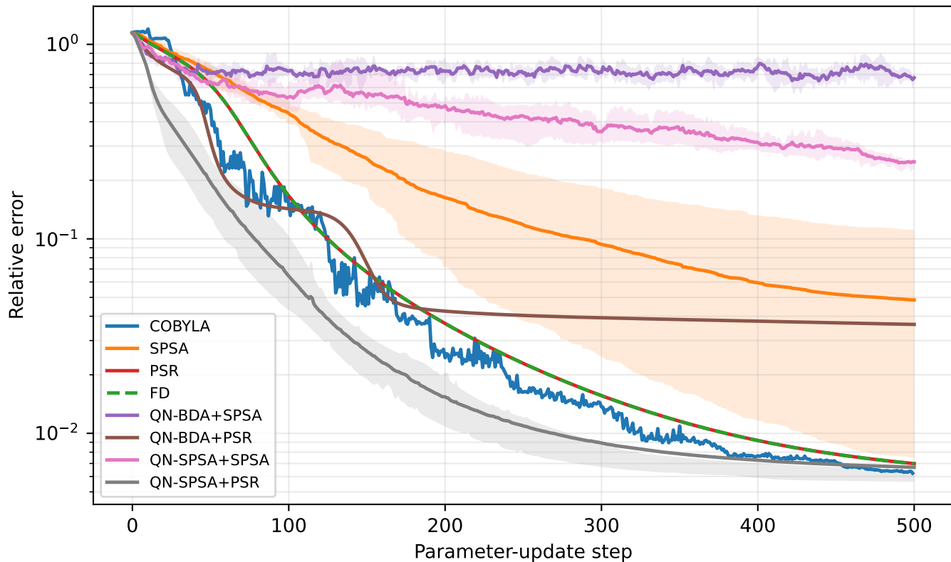
RealAmplitudes, n=12 , h=2.0 , reps=2
