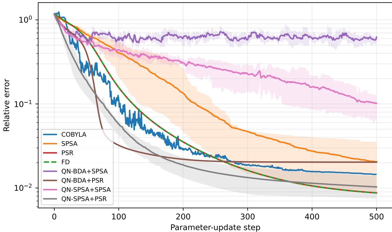
RealAmplitudes, n=9 , h=2.0 , reps=2
