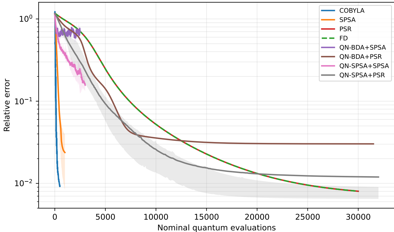
RealAmplitudes, n=10, h=2.0, reps=2
