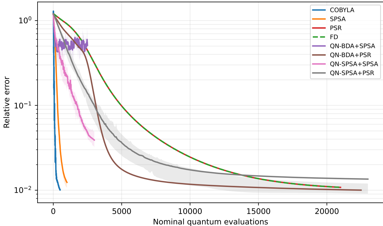
RealAmplitudes, n=7 , h=2.0 , reps=2
