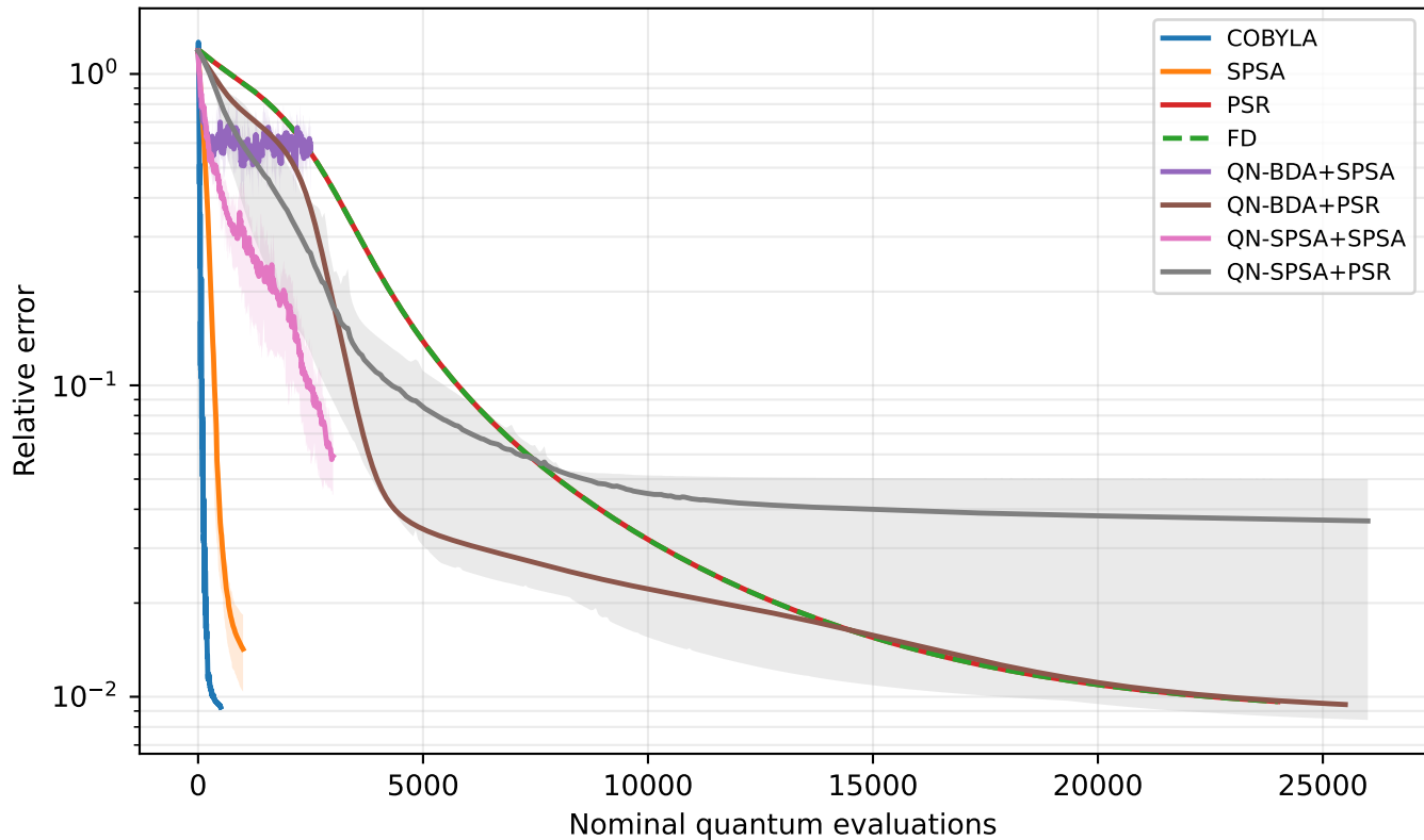
RealAmplitudes, n=8 , h=2.0 , reps=2
