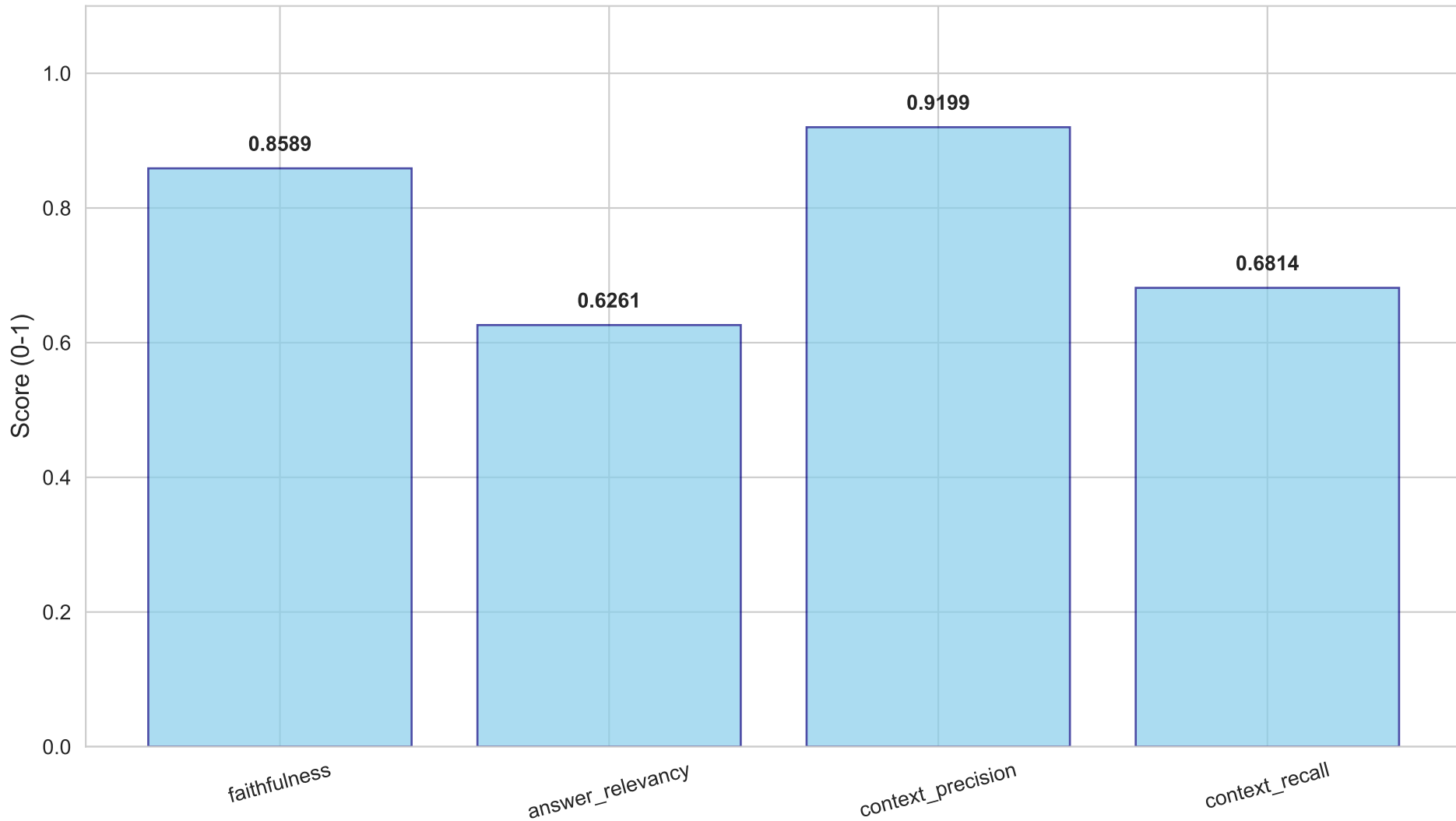
RAGAS Baseline (LLM: gpt-4o-mini | Embed: BGE-M3)
