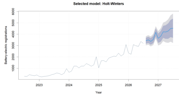
Fig. 4. Selected-model forecast with 80% and 95% intervals.
