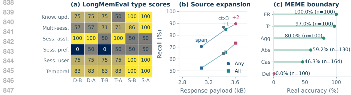
Figure 8: Additional quantitative diagnostics from the frozen ledger. (a) LongMemEval type scores for the paired Base/Align+ tracks; the directional samples have n=25/25/27 and are shown as coarse percentages. (b) Source-expansion recall versus response payload on 105 prior-error cases; this is a development diagnostic, not a held-out test. (c) MEME real task accuracy with task-specific denominators, exposing the 0% deletion boundary.
