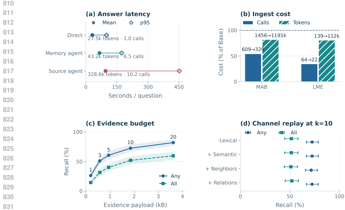
Figure 7: Operating-point diagnostics from frozen artifacts (Align+ engine; panel a over all 1,074 questions). (a) Mean-to-p95 answer latency with tokens and calls annotated; (b) paired Base→Align+ ingest cost; (c) the valid fixed-ranking retrieval-budget frontier; (d) source-only channel replay at k=10 .
