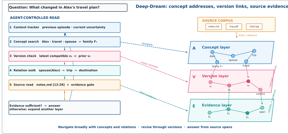
Figure 4: Deep-Dream separates agent-controlled progressive reading from a linked memory stack. The concept layer provides stable handles and relation neighborhoods; the version layer records observation-time revisions and conflicts; and the evidence layer resolves each address to an episode, chunk, and exact source span. During write , uncertain mentions may remain split and later converge; during read , the agent traverses concepts and relations, checks compatible versions, opens source evidence, and stops when the evidence gate is satisfied. Concept–version and version–evidence links make the representation revisable without changing the authority of the original span.
