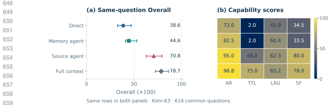
Figure 5: Same-question alignment on the n=614 questions covered by the same-model full-context reference (Kimi-K3 answerer; official macro scorer). (a) Overall scores with marginal 95% bootstrap intervals; the source-reading method scores below the reference by 7.9 points [95% CI -11.9, -3.9 ]. (b) Domain profiles: the reference’s margin concentrates in TTL, while the source-reading method matches or exceeds the reference on AR, LRU, and SF.
