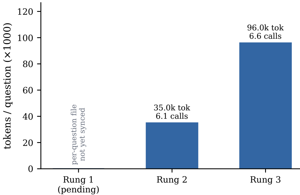
Figure 3: Per-question compute by rung, recomputed deterministically from run logs (tokens and LLM calls, mean over the 767 questions; v2 engine). Rung 1’s per-question log was not part of the artifact sync; its position is marked pending rather than estimated. The top rung buys its accuracy with an agentic verification loop; the cost accounting is part of the result, not a footnote.
