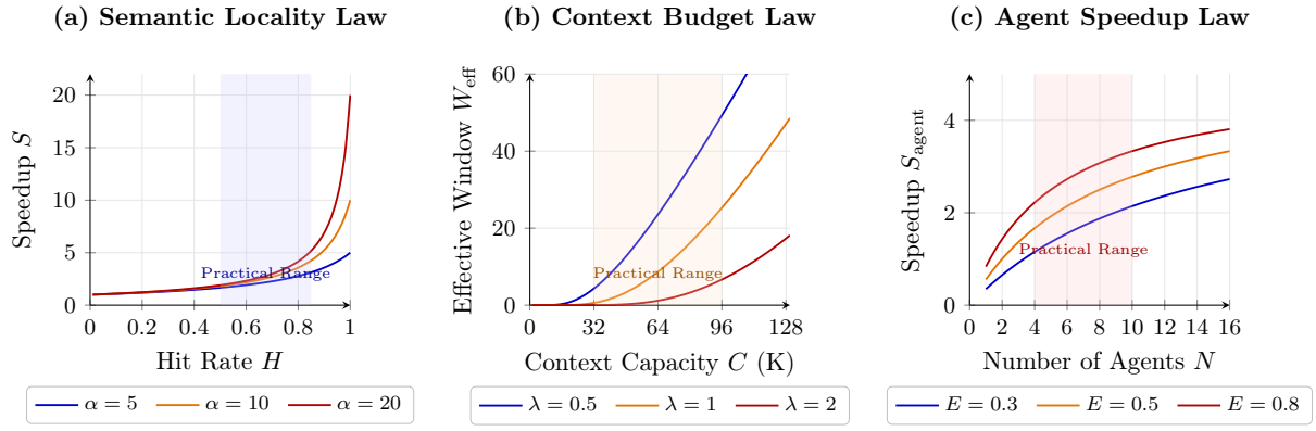
Figure 7: Characteristic curves of three quantitative laws. (a) Semantic Locality Law: S = 1/((1 - H) + H/\alpha) . (b) Context Budget Law: W_{\text{eff}} = C \cdot e^{-\lambda C_0/C} . (c) Agent Speedup Law: S = 1/((1 - F) + F/(NE)) with F = 0.8 . Shaded areas indicate typical operating ranges.
