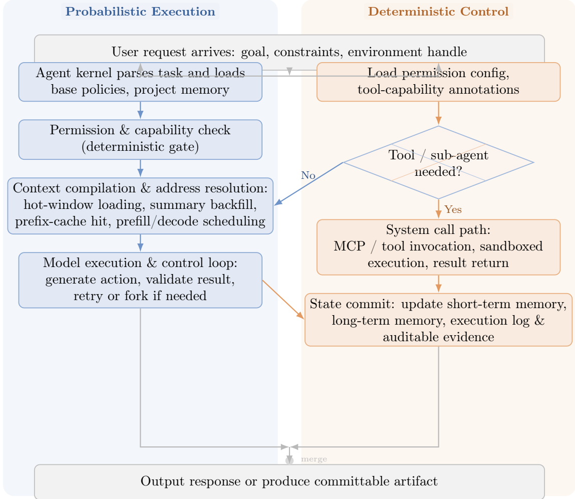
Figure 6: Request flow through the model-native computing architecture as a dual-plane swim-lane diagram. Blue nodes belong to the probabilistic execution plane; orange nodes belong to the deterministic control plane. The split-coloured diamond represents the control-plane decision that gates both paths. Grey boxes span both planes.
