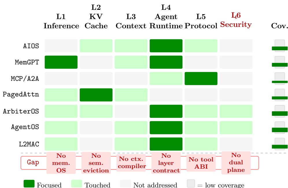
Figure 3: Coverage of ICA layers by existing works. The bottom row identifies the specific gap in each layer that no single work has addressed. The rightmost bars show per-system coverage (proportion of layers addressed). L6 Security (marked ↓) is the least-covered layer overall.
