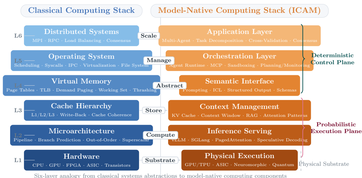
Figure 2: Layer comparison between the classical computing stack and the model-native computing stack.
