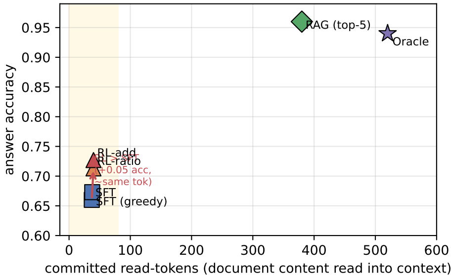
Accuracy-per-read-token frontier (held-out n=150, leakage-
