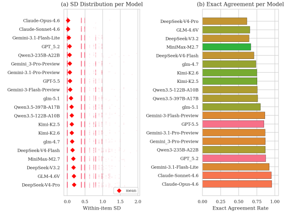
Figure 19: Model-level within-sample consistency. (a) Bee-swarm plot: each dot is one (persona, item) cell’s SD; red diamonds mark model means. Models ordered by mean SD (ascending). (b) Exact agreement rate per model, colored by vendor family.
