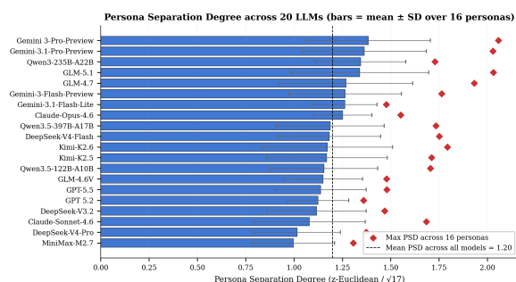
Figure 8: Persona Separation Degree (mean across 16 MBTI personas, bars; max, diamonds; SD as error bars) per model.
