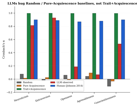
Figure 18: Cronbach’s \alpha per IPIP Big Five domain for Random, Pure Acquiescence, Trait+Acquiescence, LLM observed, and the human Johnson (2014) baseline.
