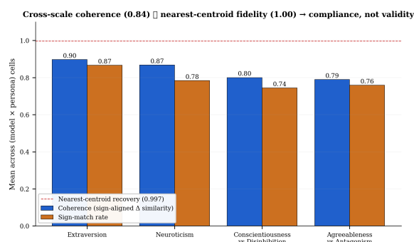
Figure 10: Cross-scale coherence (blue) and sign-match rate (orange) per construct. Far below nearest-centroid fidelity (dashed red).
