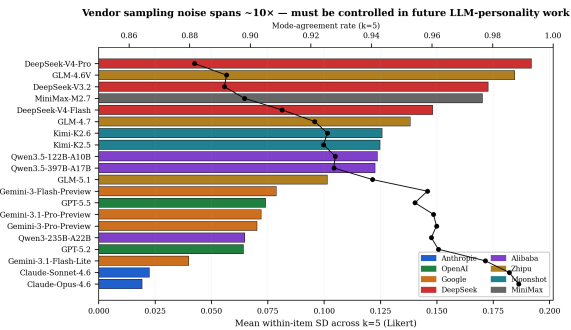
Figure 20: Within-sample stability across k = 5 repeats per model (Likert items). Bars: mean within-item SD coloured by vendor family. Line: mode-agreement rate on the secondary axis. Vendor sampling noise spans \approx 10\times .
