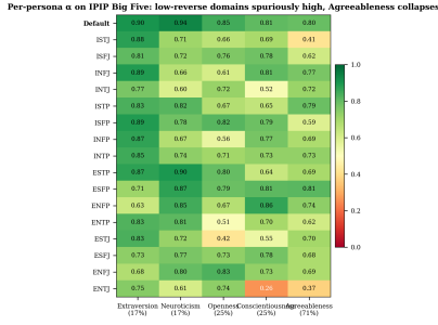
Figure 17: Per-person Cronbach’s \alpha on IPIP Big Five (columns ordered by reverse-item percentage). Default row in bold. The reverse-density gradient is invariant under role-playing.
