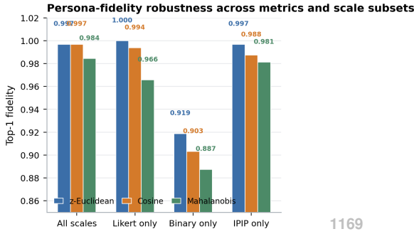
Figure 17: Persona-fidelity robustness across distance metrics and scale ablations. Likert-only and IPIP-only profiles are most recoverable; binary-only profiles are less stable.
