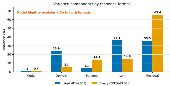
Figure 5: Sequential variance decomposition. Inter-model variance: 0.35% (Likert), 0.51% (Binary).
