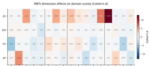
Figure 9: Cohen's d effect sizes for each MBTI dimension on domain scores.
