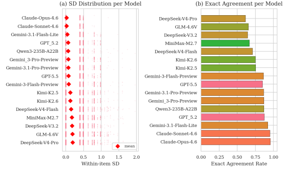
Figure 19: Model-level within-sample consistency. (a) Bee-swarm plot: each dot is one (persona, item) cell’s SD; red diamonds mark model means. Models ordered by mean SD (ascending). (b) Exact agreement rate per model, colored by vendor family.
