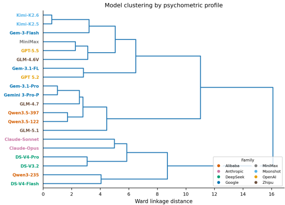
Figure 8: Hierarchical clustering of 20 models by z-scored Default domain profiles. Models do not cluster cleanly by vendor.
