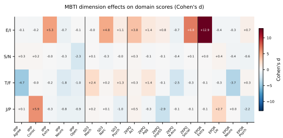
Figure 10: Cohen's d effect sizes for each MBTI dimension on domain scores.
