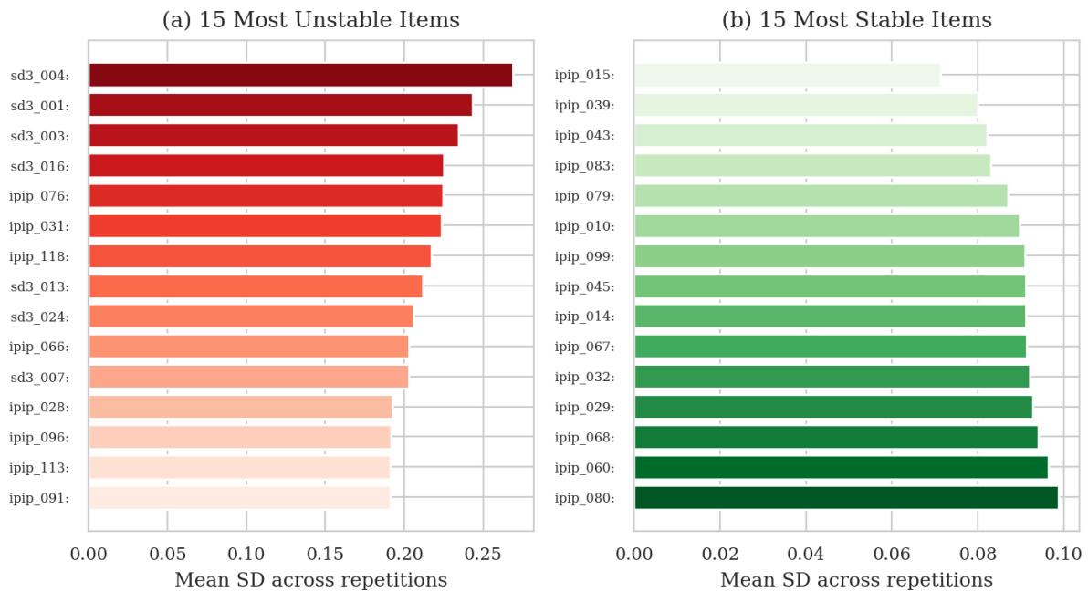
Figure 22: Item-level stability ranking (Likert items). (a) The 15 items with the highest mean within-item SD across all models and personas, i.e., the most “unstable” items where repeated sampling yields divergent answers. (b) The 15 most stable items. Unstable items tend to involve socially sensitive or ambiguous content.
