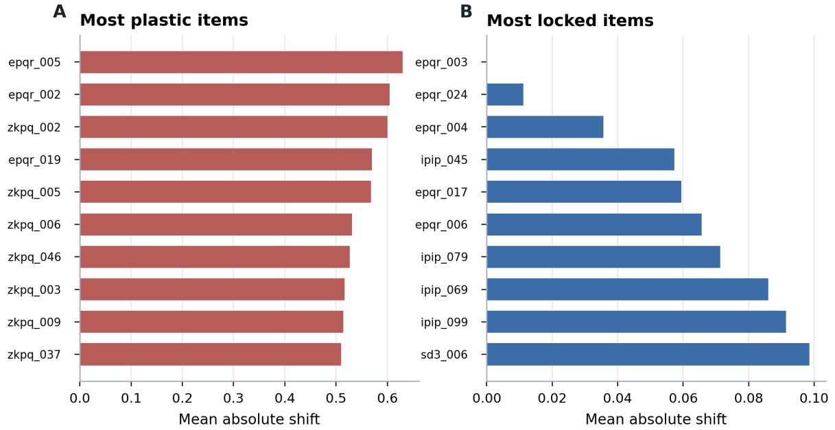
Figure 15: Most plastic and most locked items under MBTI persona steering. Plastic items are mostly activity, sociability, and rule-following items; locked items are concentrated in safety- and morality-sensitive content.
