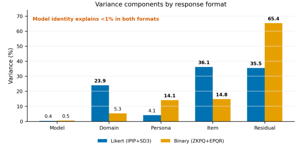
Figure 5: Sequential variance decomposition. Inter-model variance: 0.35% (Likert), 0.51% (Binary).
