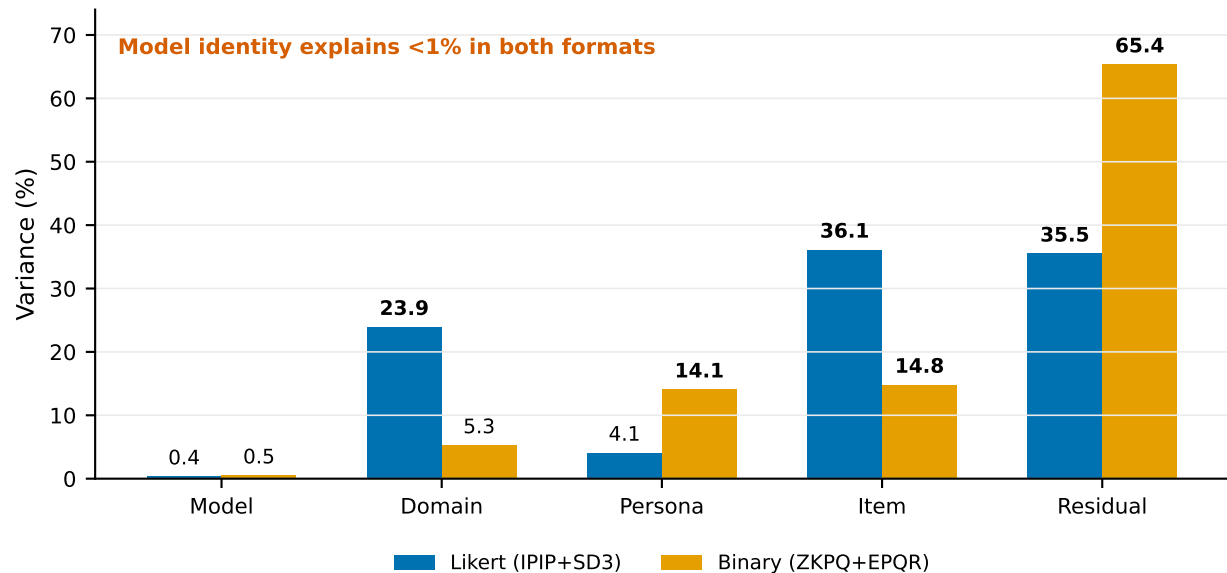
Variance components by response format
