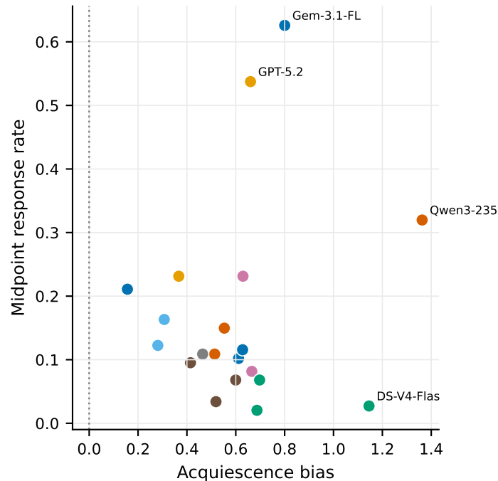
(A) Response style map
