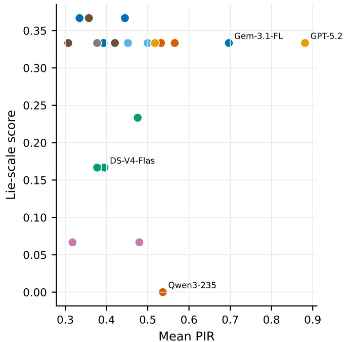
(B) Inconsistency vs social desirability
